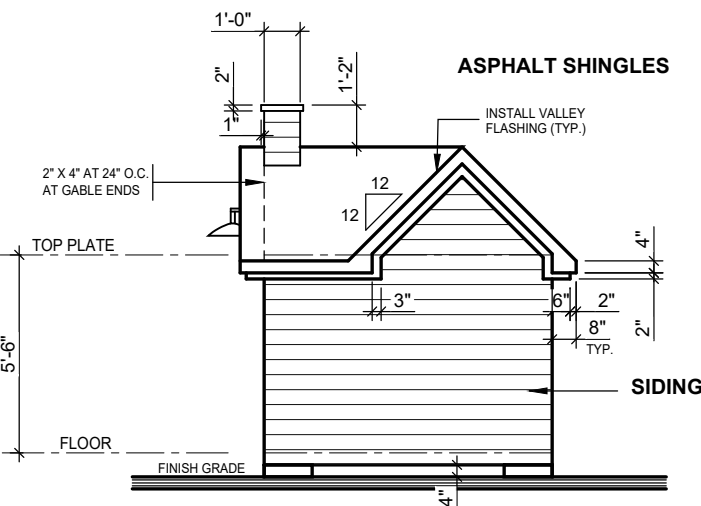
REAR ELEVATION
