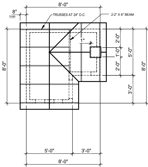
ROOF PLAN
